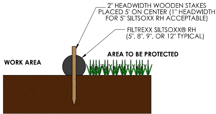
SECTION VIEW
