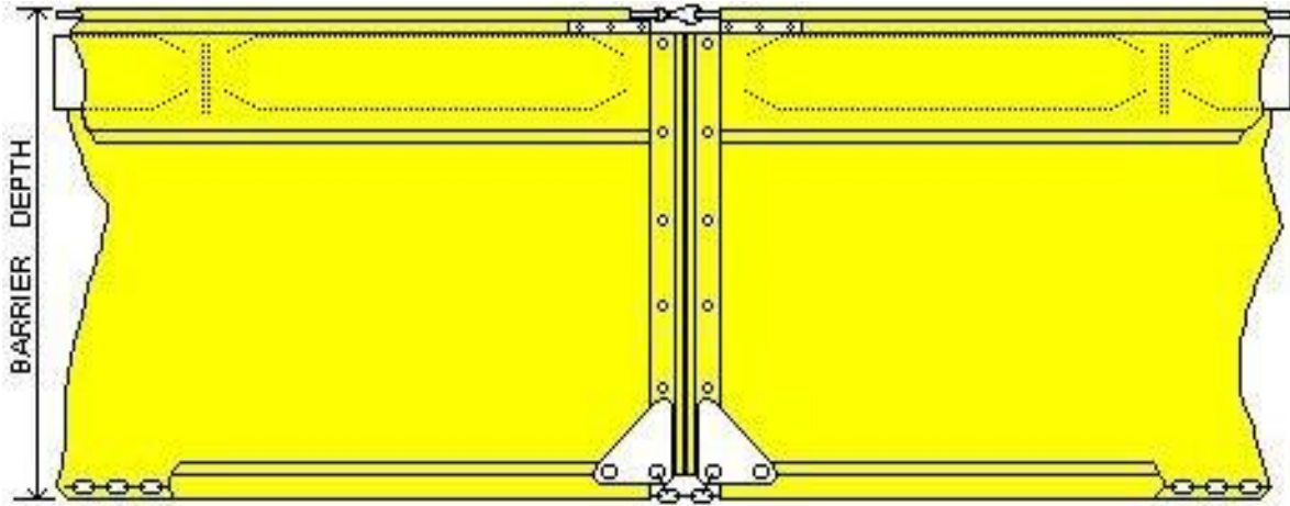
Tough-Guy® Floating Turbidity Barrier Type 2.DOT
