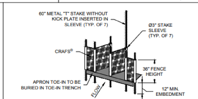
48" ISOMETRIC VIEW
