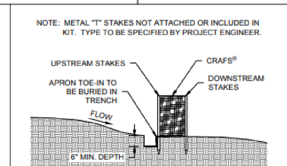
PROFILE VIEW
