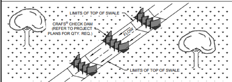
CHECK DAM - PERSPECTIVE VIEW
