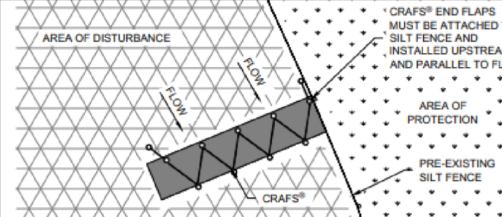
J-HOOK - TOP VIEW
