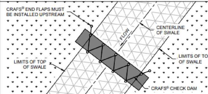
CHECK DAM - TOP VIEW
