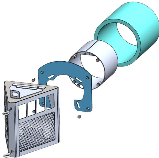
StormRing Exploded View
